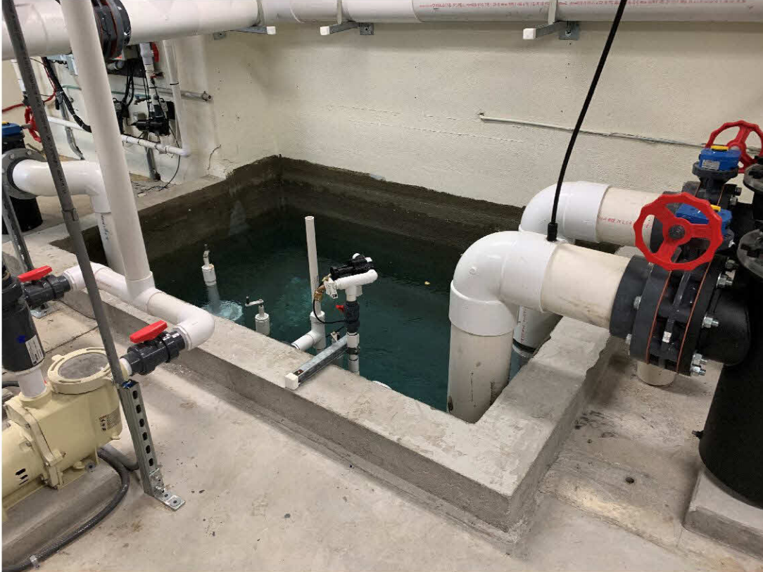
New sump with circulation intakes and auto-fill
